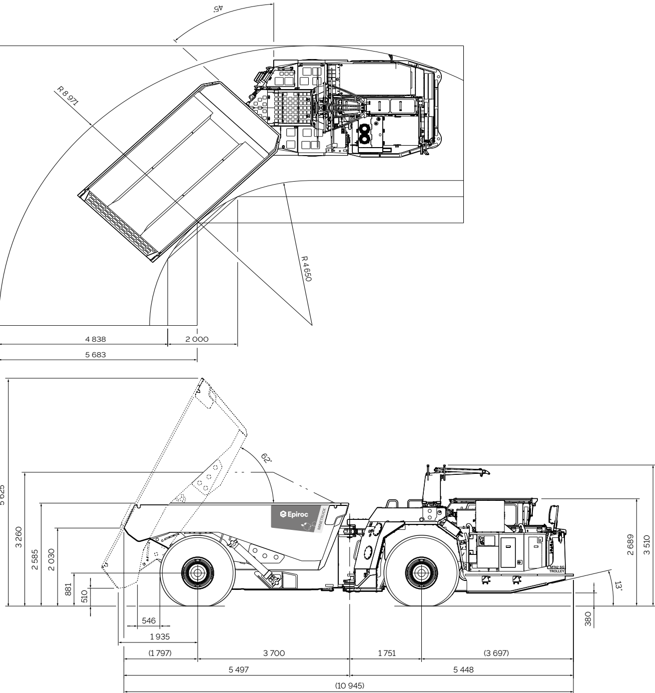
All dimensions are shown in millimeters (mm). Dimensions and calculations shown are based on standard vehicle configuration with 30 mm tire deflection, unloaded.
