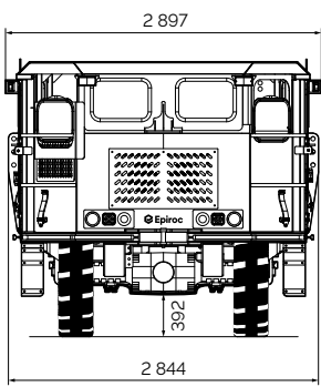
Rear view of Terrah TS100 PEC
