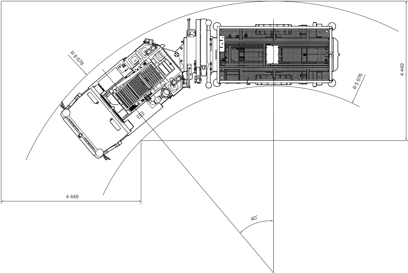
Turning radius of Terrah TS100 SCL
