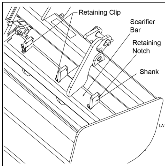
Figure 4. Scarifier Shanks
